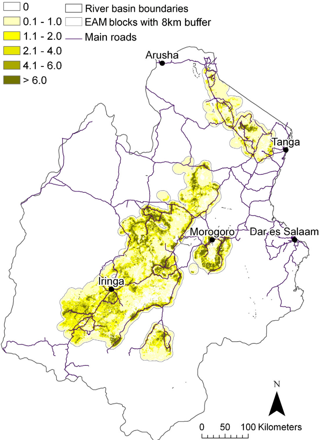
Fig. 4. Total annual value of charcoal produced (TSH*1000 per ha per year).
