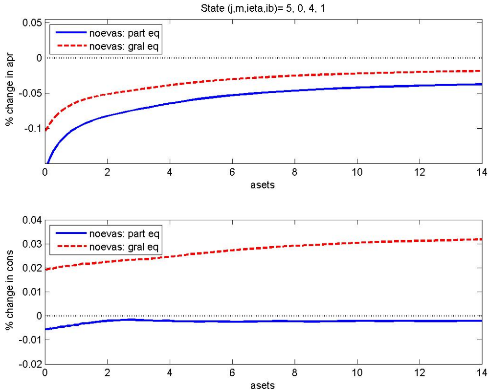
Figure 12: No evasion. Change in policy functions. Partial and general equilibrium.
